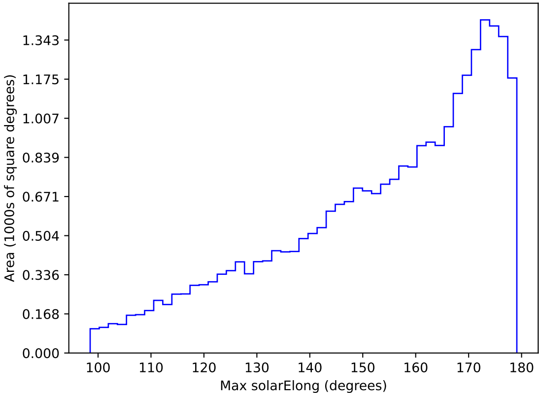
ddf_loaded_half_fl4_v3.4_10yrs All sky g band: Max solarElong
