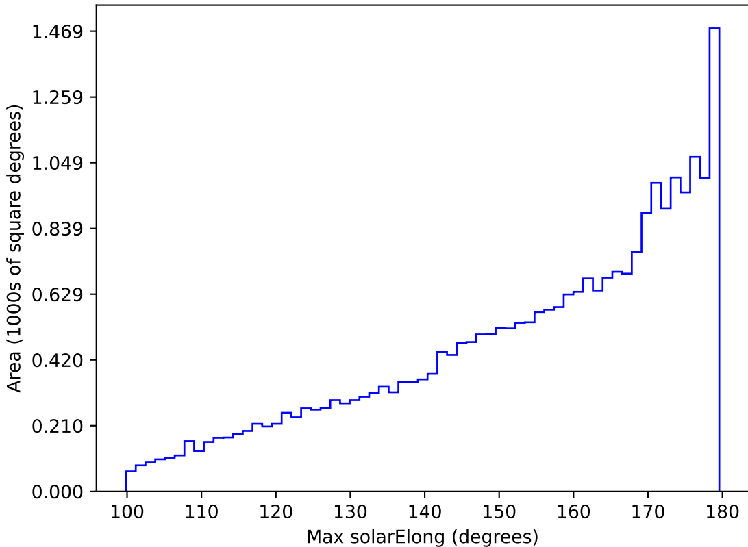
ddf_loaded_half_fl4_v3.4_10yrs All sky all bands: Max solarElong
