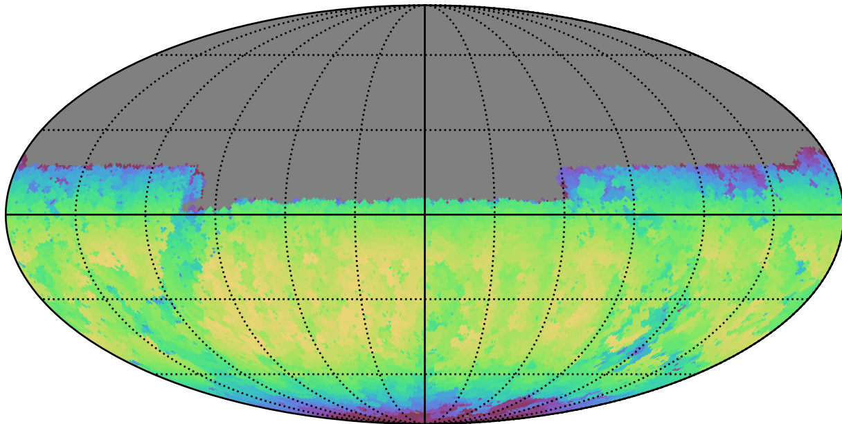
ddf_loaded_half_fl4_v3.4_10yrs Yr 1 y band: Max skyBrightness
