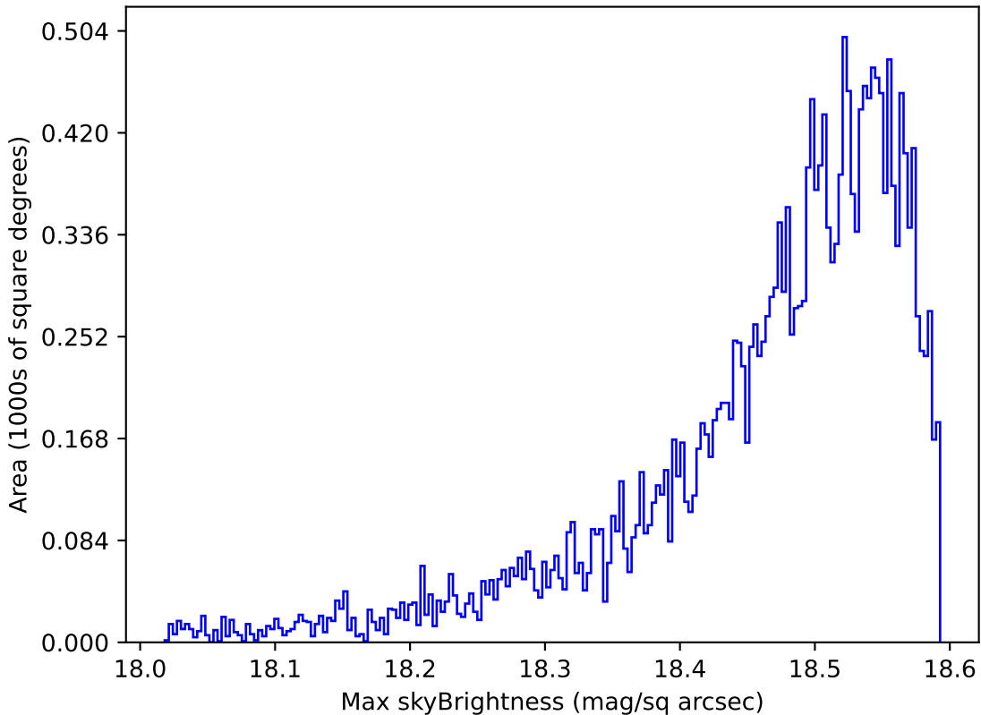
ddf_loaded_half_fl4_v3.4_10yrs Yr 1 y band: Max skyBrightness
