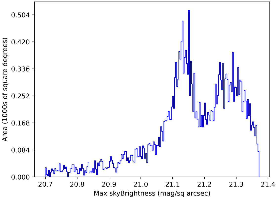
ddf_loaded_half_fl4_v3.4_10yrs Yr 1 r band: Max skyBrightness
