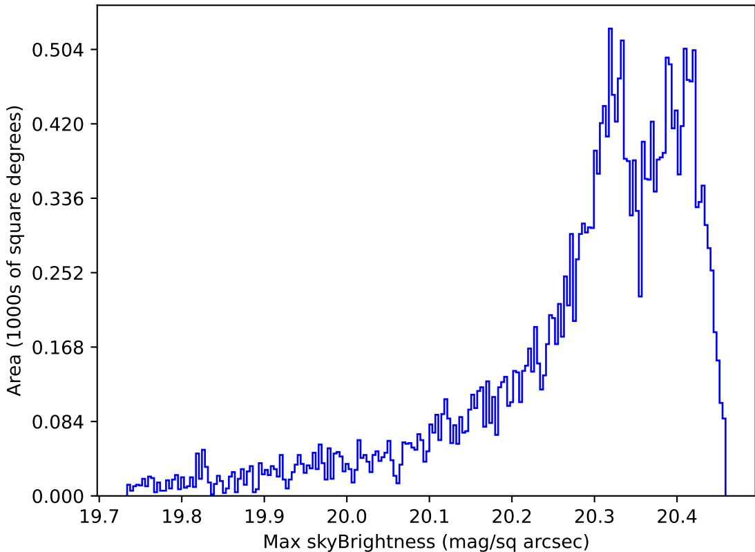
ddf_loaded_half_fl4_v3.4_10yrs Yr 1 i band: Max skyBrightness
