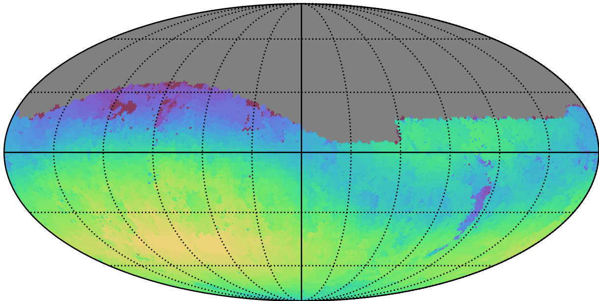
ddf_loaded_half_fl4_v3.4_10yrs Yr 1 g band: Max skyBrightness
