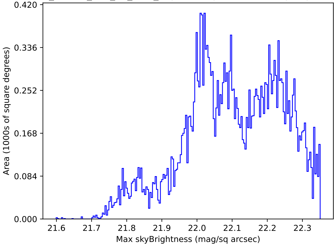
ddf_loaded_half_fl4_v3.4_10yrs Yr 1 g band: Max skyBrightness
