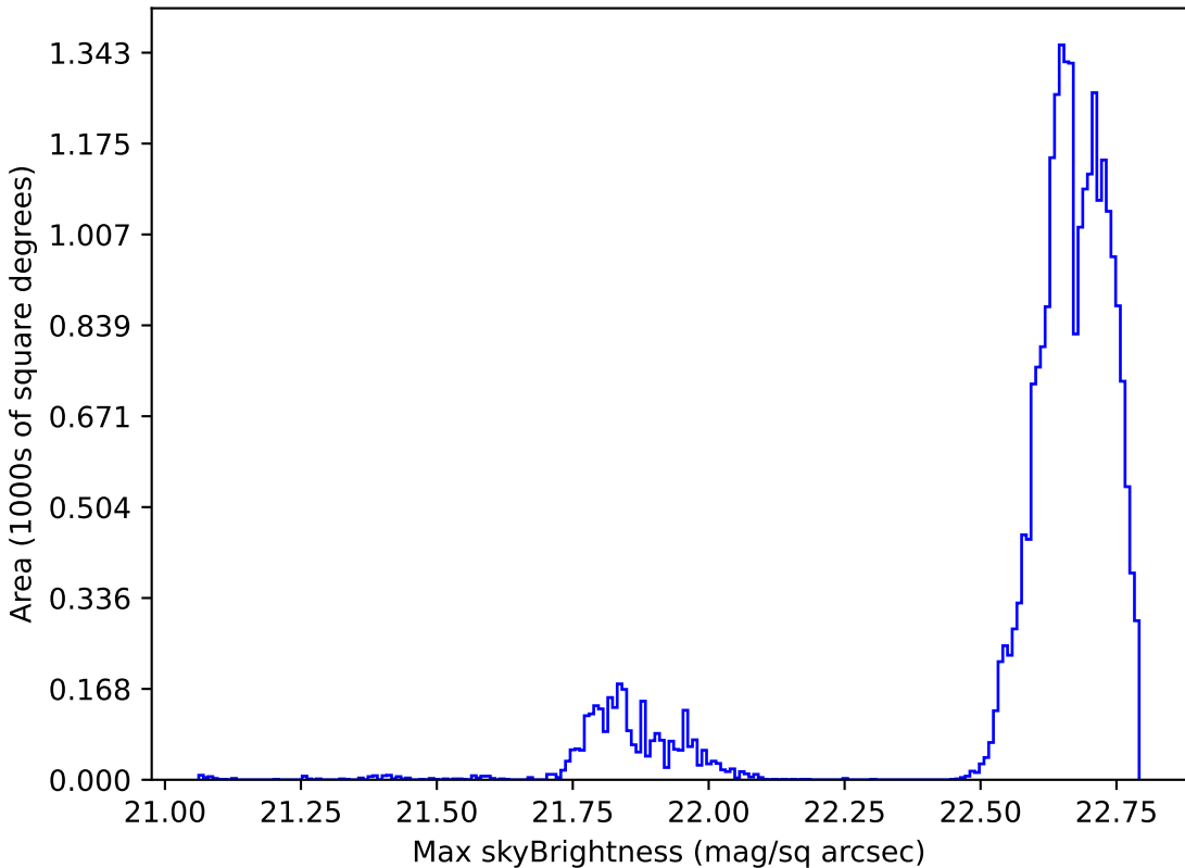
ddf_loaded_half_fl4_v3.4_10yrs Yr 1 all bands: Max skyBrightness
