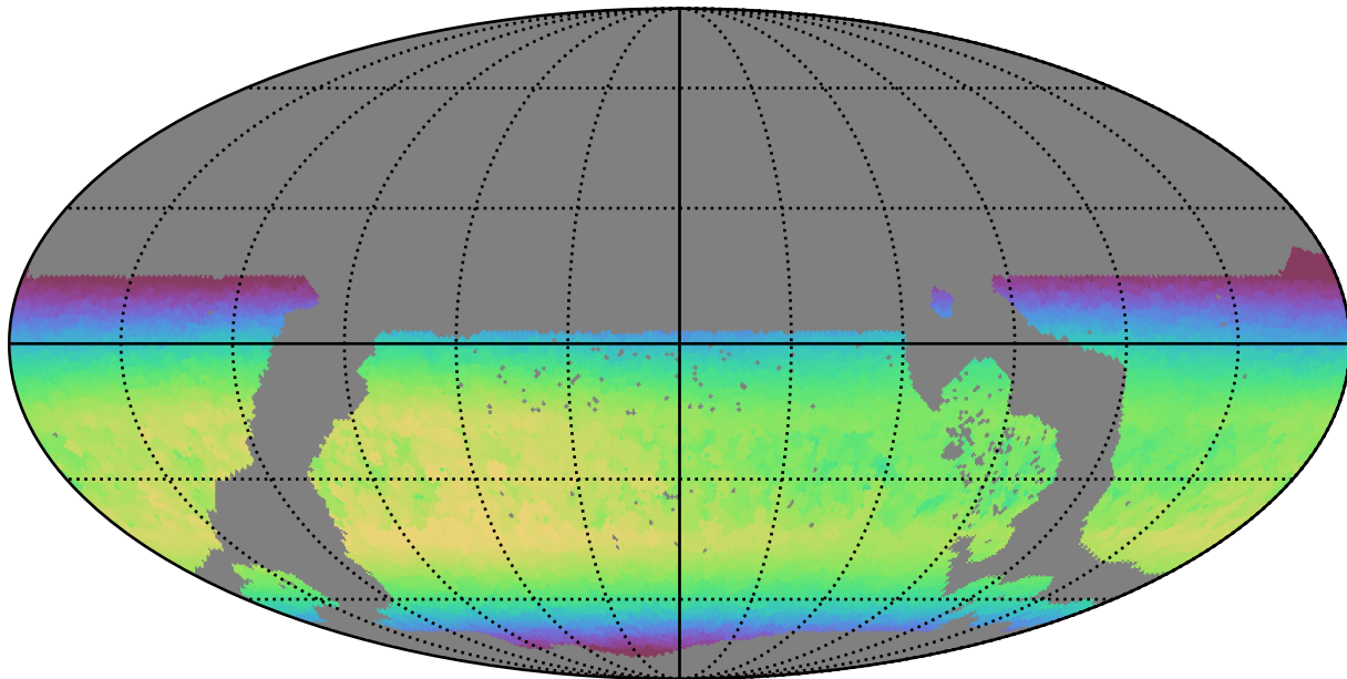
ddf_loaded_half_fl4_v3.4_10yrs WFD z band: Max skyBrightness
