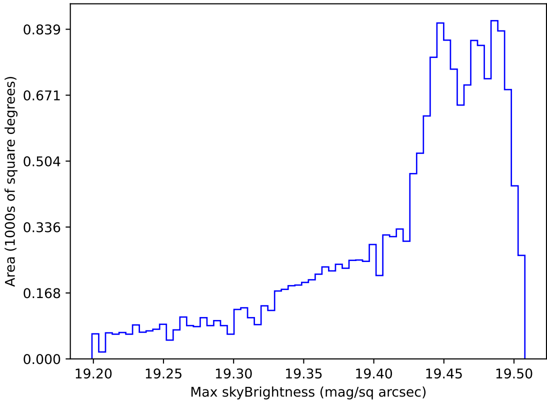
ddf_loaded_half_f14_v3.4_10yrs WFD z band: Max skyBrightness
