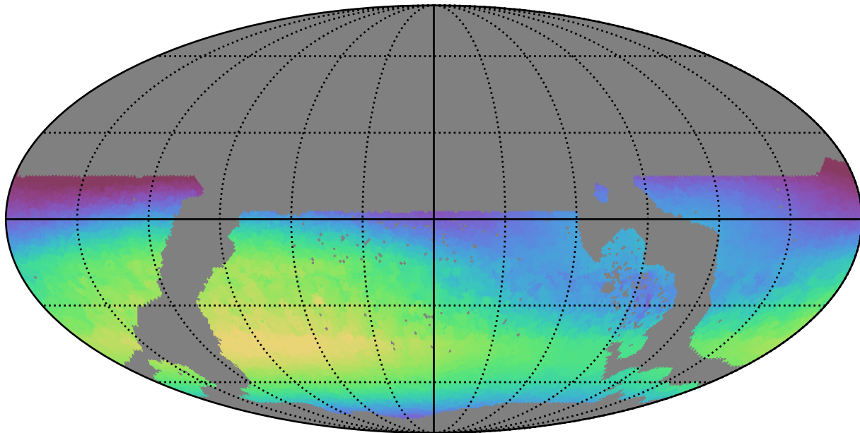
ddf_loaded_half_fl4_v3.4_10yrs WFD u band: Max skyBrightness
