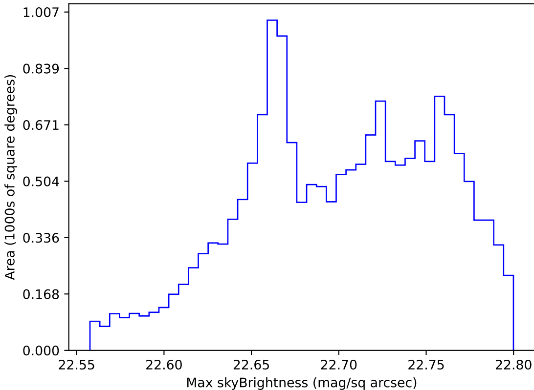
ddf_loaded_half_fl4_v3.4_10yrs WFD u band: Max skyBrightness
