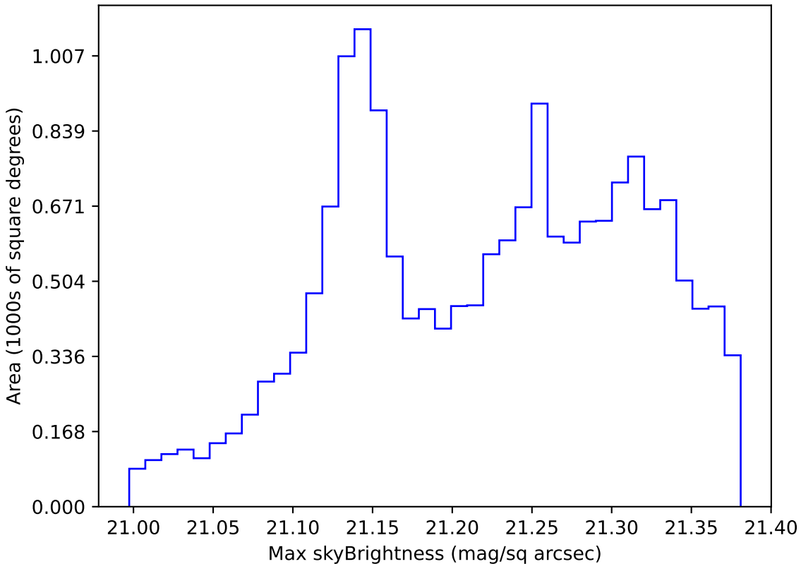
ddf_loaded_half_fl4_v3.4_10yrs WFD r band: Max skyBrightness
