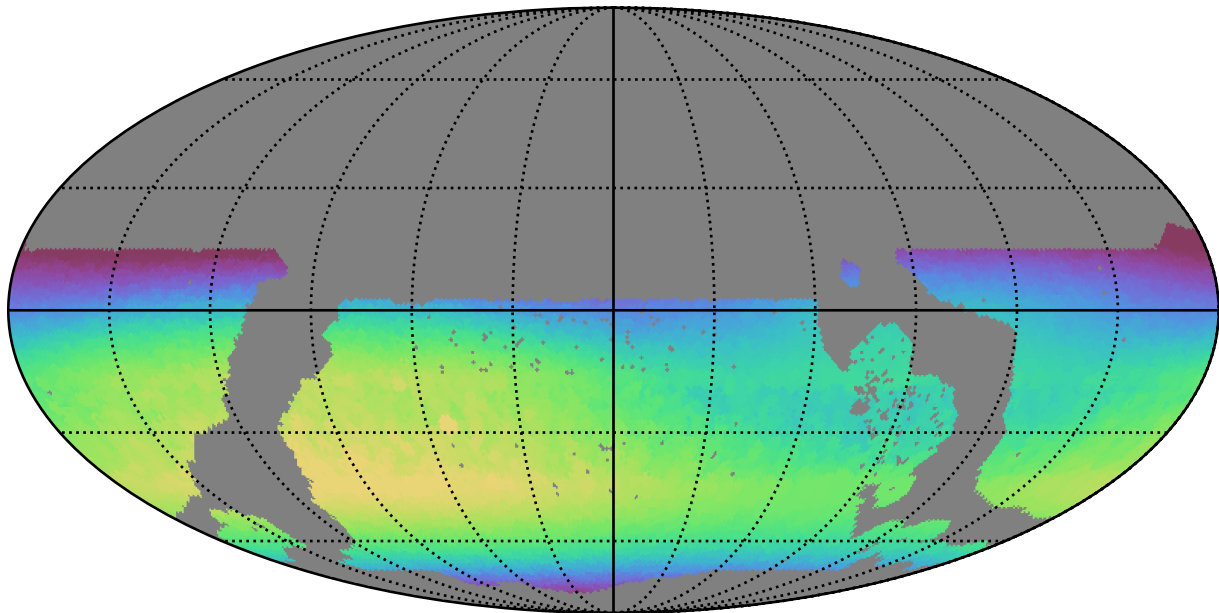
ddf_loaded_half_fl4_v3.4_10yrs WFD i band: Max skyBrightness
