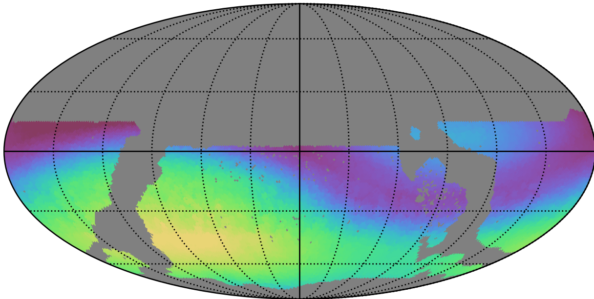
ddf_loaded_half_fl4_v3.4_10yrs WFD g band: Max skyBrightness
