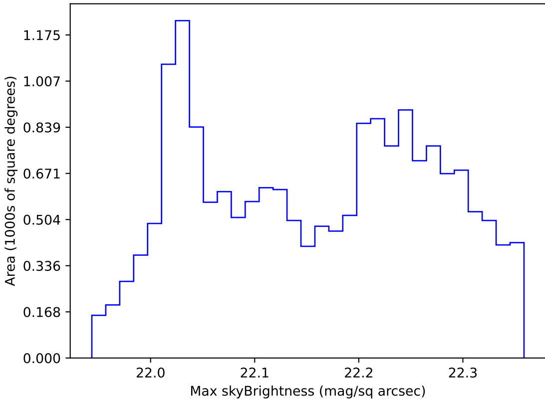
ddf_loaded_half_fl4_v3.4_10yrs WFD g band: Max skyBrightness
