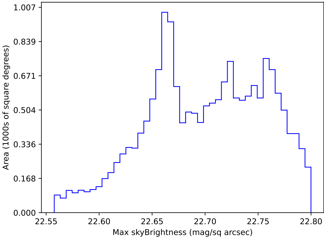
ddf_loaded_half_fl4_v3.4_10yrs WFD all bands: Max skyBrightness
