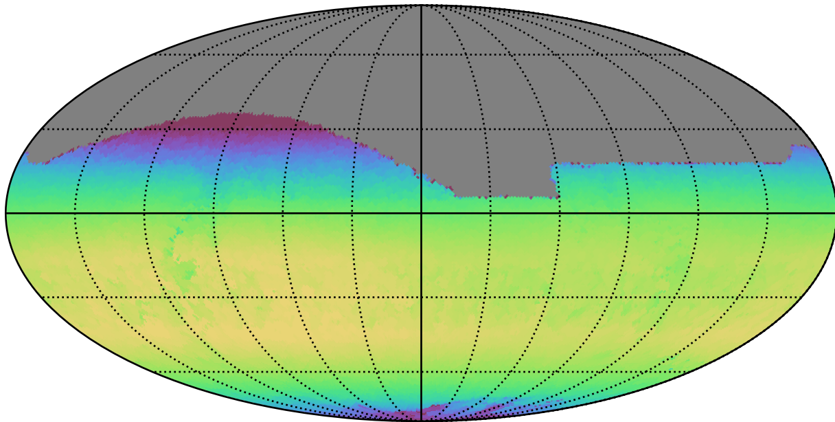
ddf_loaded_half_fl4_v3.4_10yrs All sky z band: Max skyBrightness
