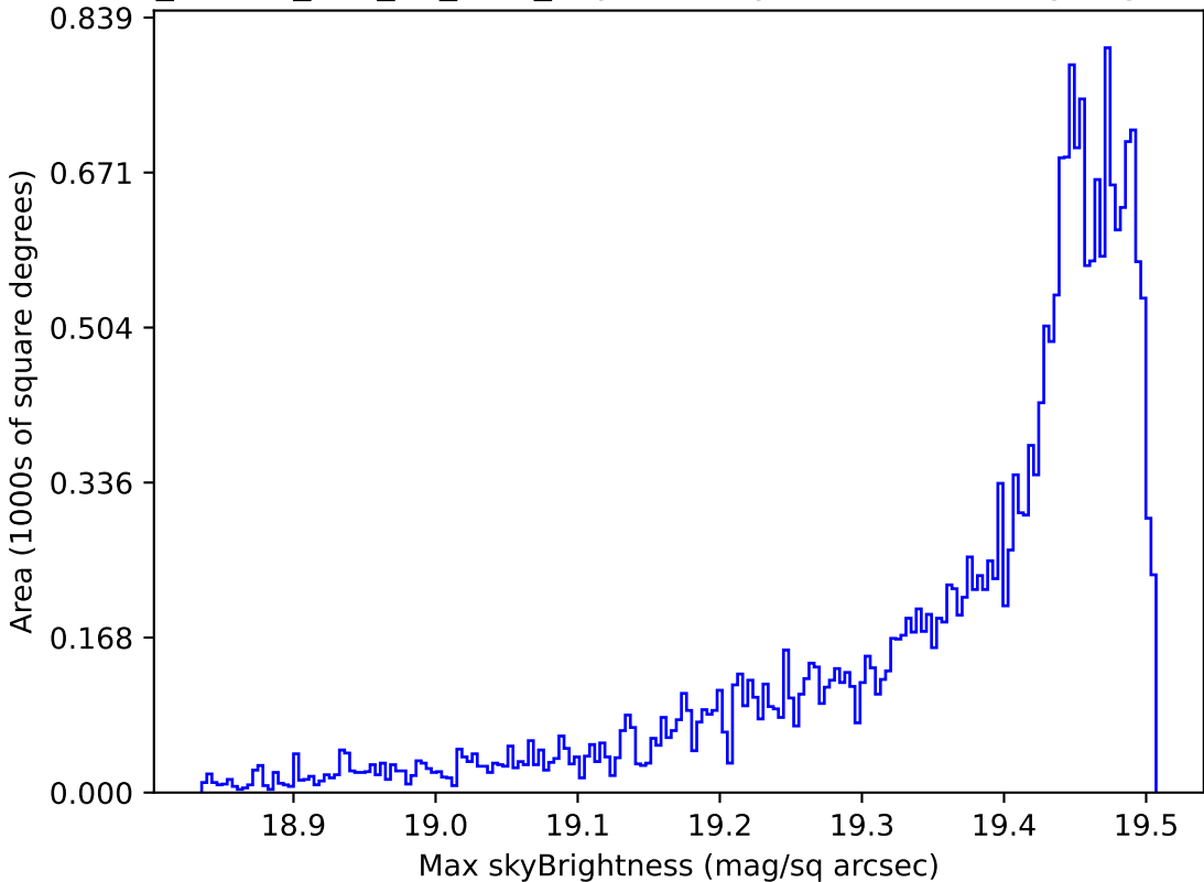
ddf_loaded_half_fl4_v3.4_10yrs All sky z band: Max skyBrightness
