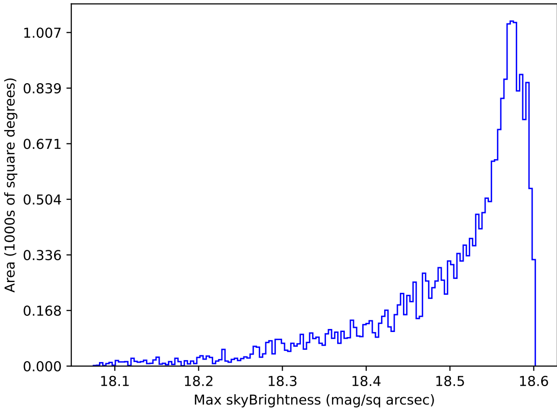
ddf_loaded_half_fl4_v3.4_10yrs All sky y band: Max skyBrightness
