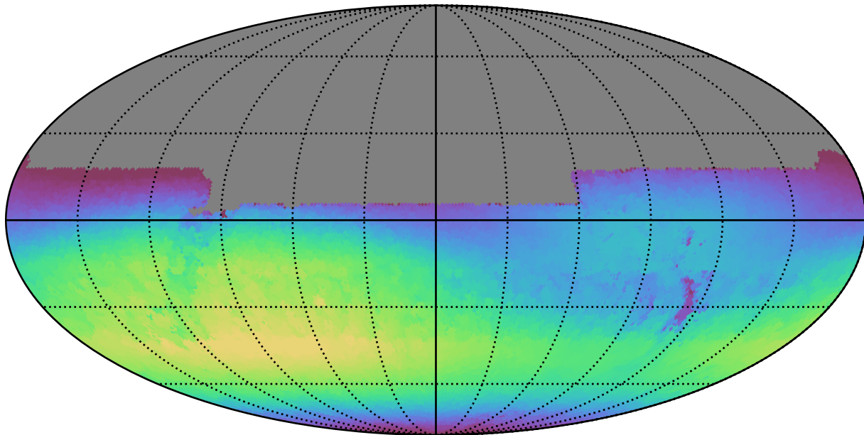
ddf_loaded_half_fl4_v3.4_10yrs All sky u band: Max skyBrightness
