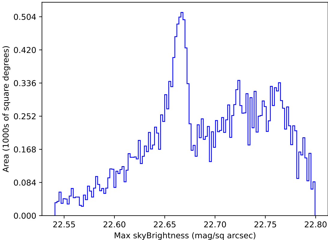
ddf_loaded_half_fl4_v3.4_10yrs All sky u band: Max skyBrightness
