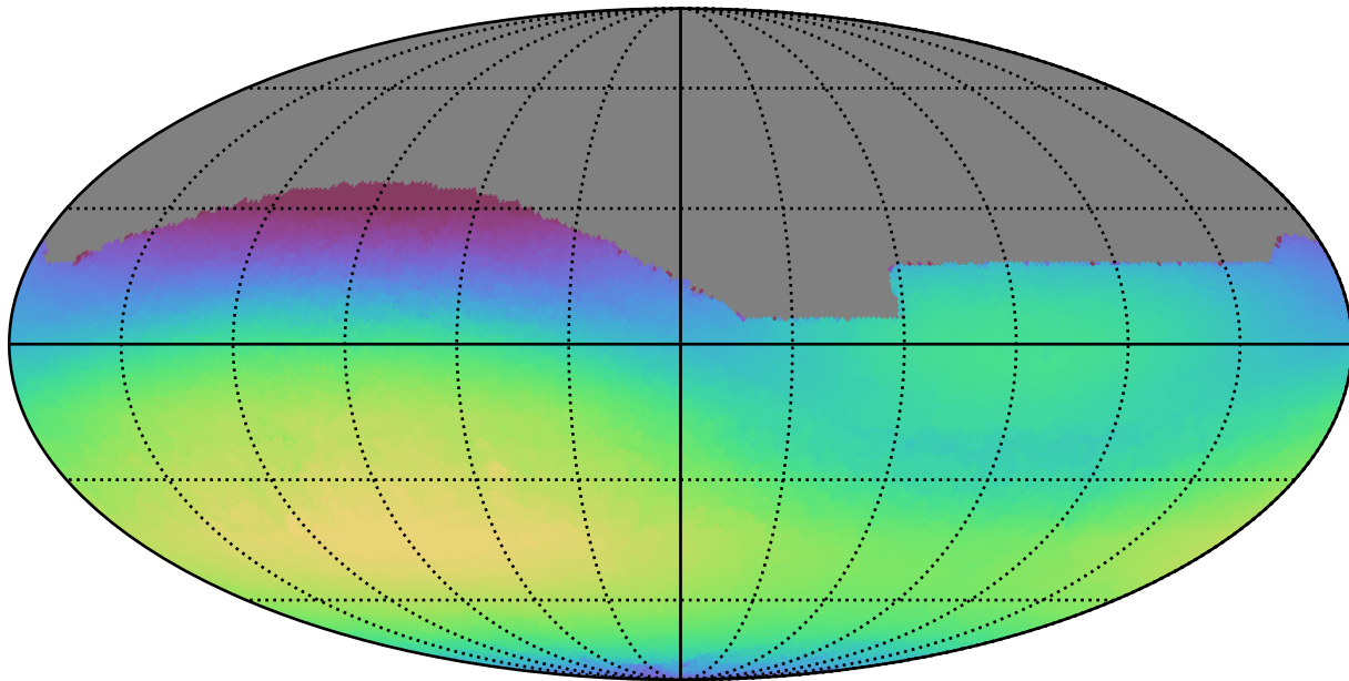
ddf_loaded_half_fl4_v3.4_10yrs All sky r band: Max skyBrightness
