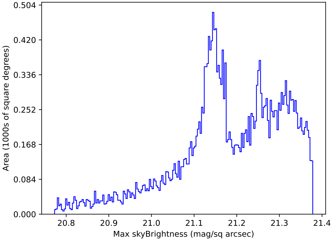
ddf_loaded_half_fl4_v3.4_10yrs All sky r band: Max skyBrightness
