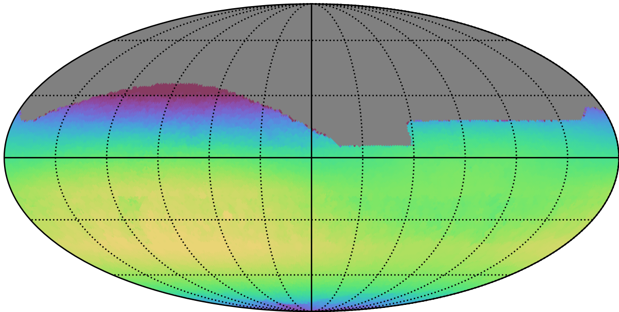
ddf_loaded_half_fl4_v3.4_10yrs All sky i band: Max skyBrightness
