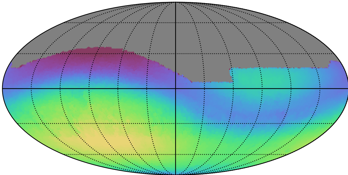
ddf_loaded_half_fl4_v3.4_10yrs All sky g band: Max skyBrightness
