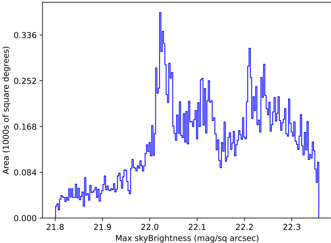
ddf_loaded_half_fl4_v3.4_10yrs All sky g band: Max skyBrightness
