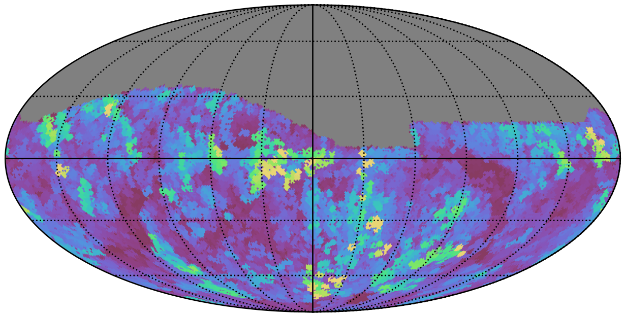
ddf_loaded_half_fl4_v3.4_10yrs Yr 1 z band: Max seeingGeom
