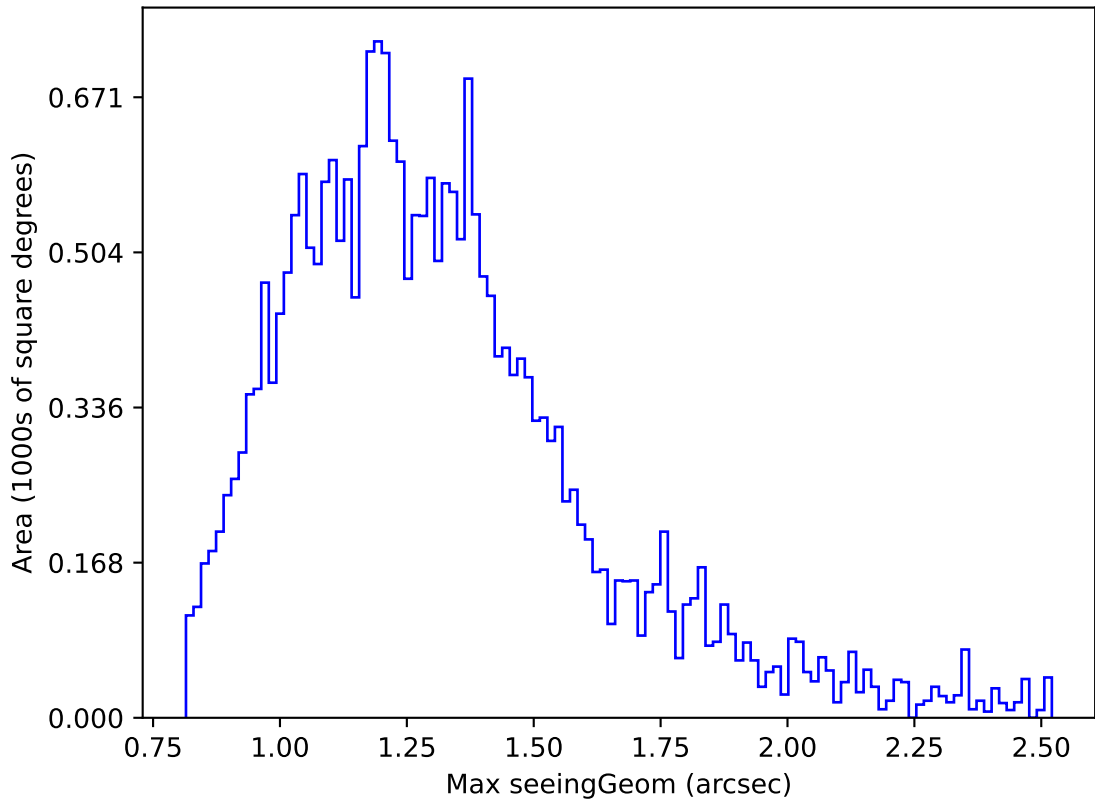
ddf_loaded_half_fl4_v3.4_10yrs Yr 1 z band: Max seeingGeom
