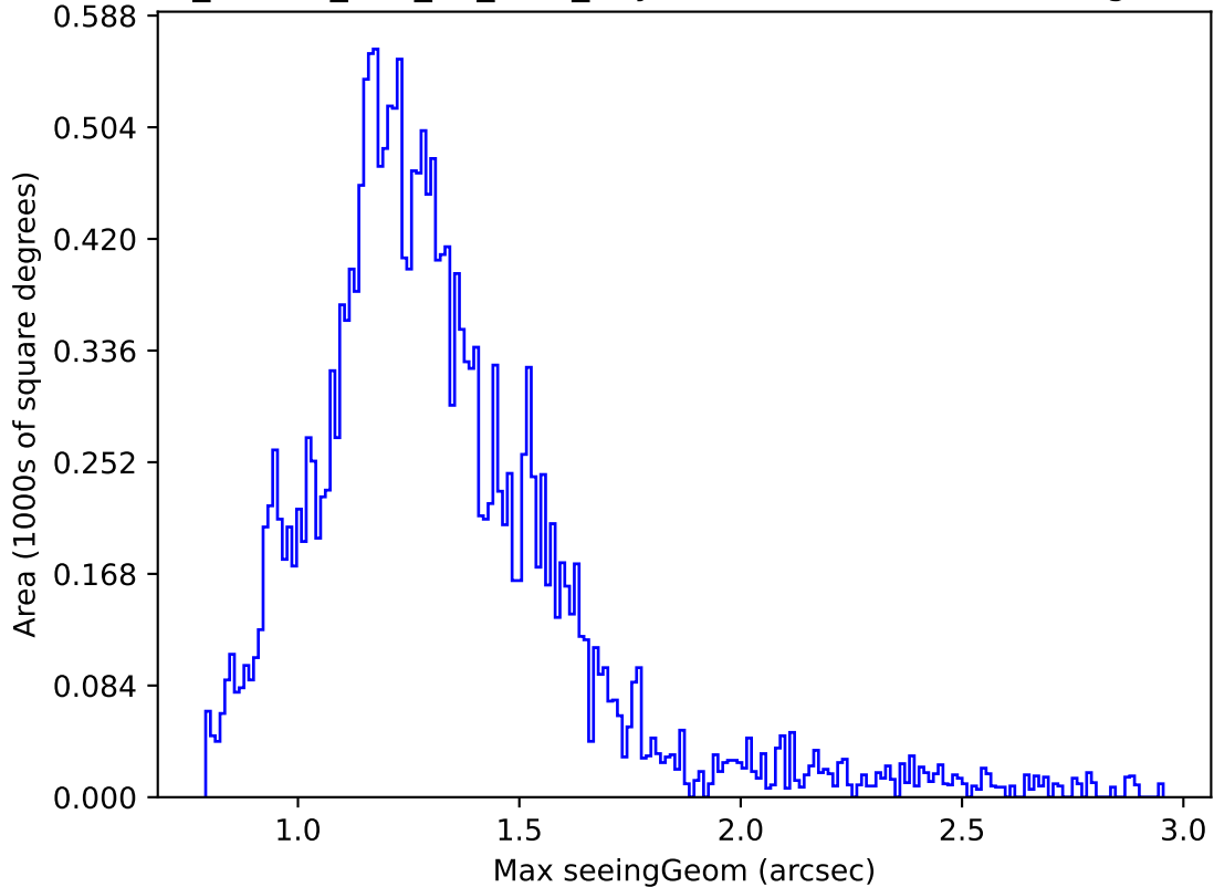
ddf_loaded_half_fl4_v3.4_10yrs Yr 1 u band: Max seeingGeom
