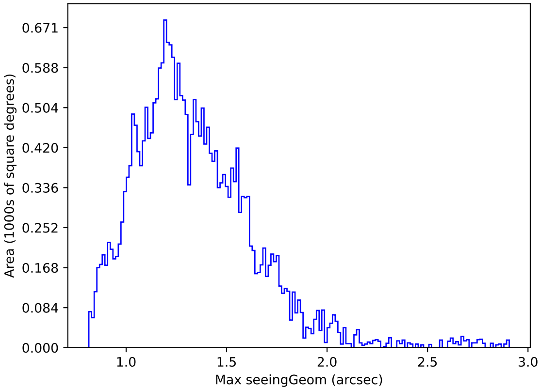
ddf_loaded_half_fl4_v3.4_10yrs Yr 1 r band: Max seeingGeom
