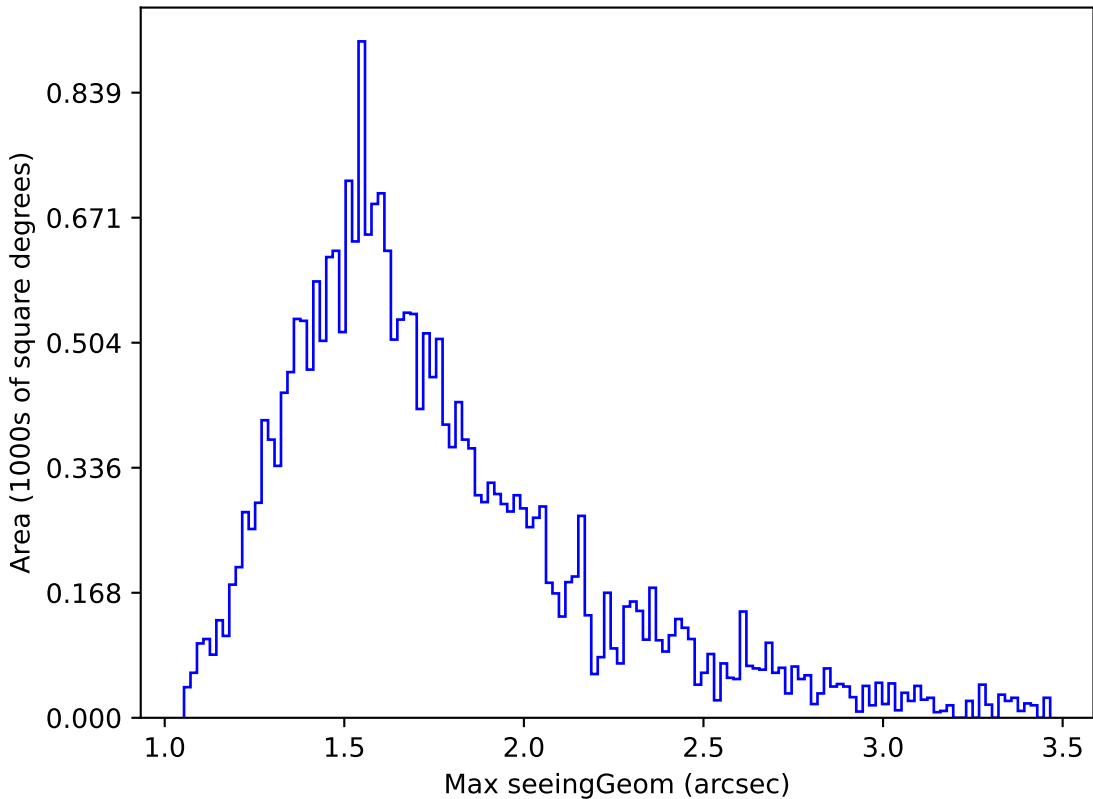
ddf_loaded_half_fl4_v3.4_10yrs Yr 1 all bands: Max seeingGeom
