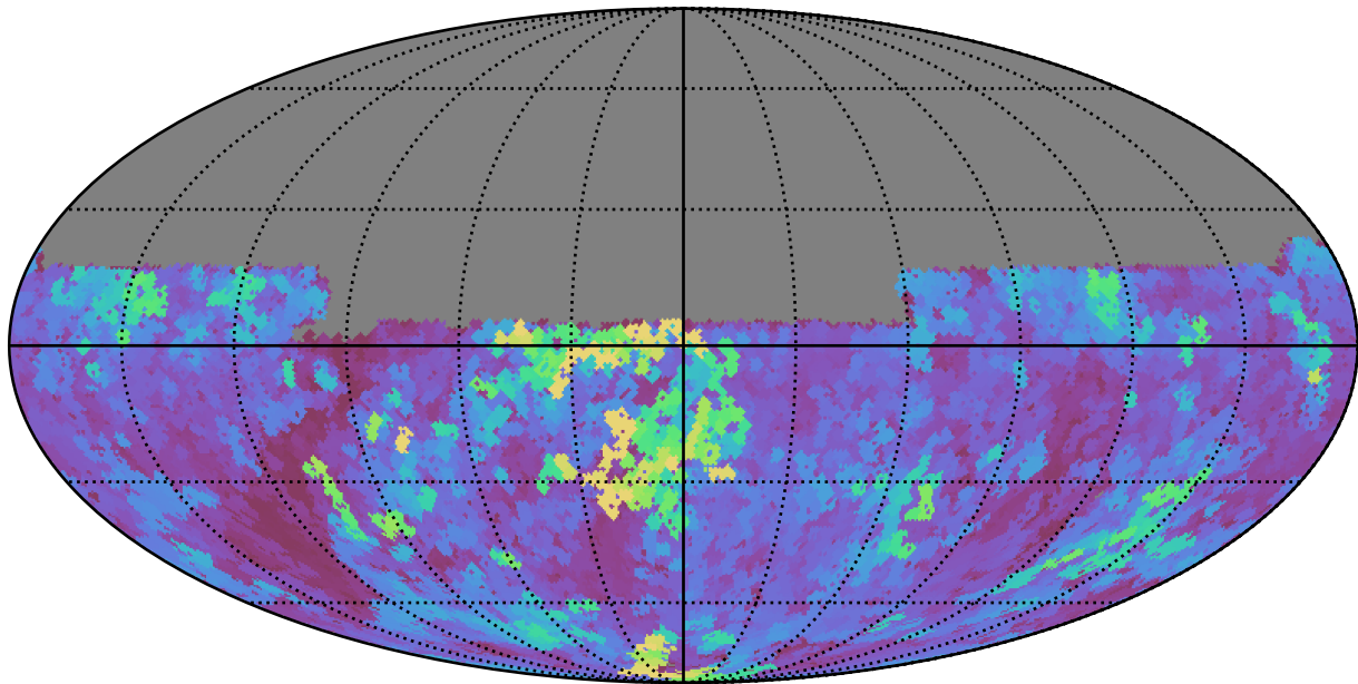
ddf_loaded_half_fl4_v3.4_10yrs Yr 1 y band: Max seeingEff
