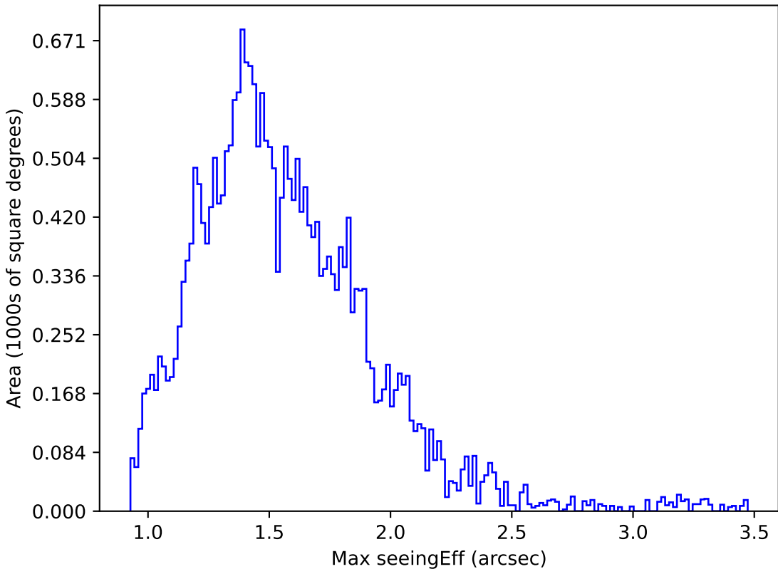
ddf_loaded_half_fl4_v3.4_10yrs Yr 1 r band: Max seeingEff
