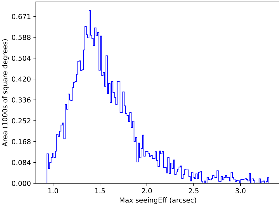
ddf_loaded_half_fl4_v3.4_10yrs Yr 1 i band: Max seeingEff
