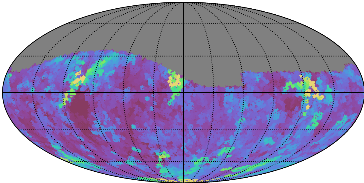
ddf_loaded_half_fl4_v3.4_10yrs Yr 1 g band: Max seeingEff
