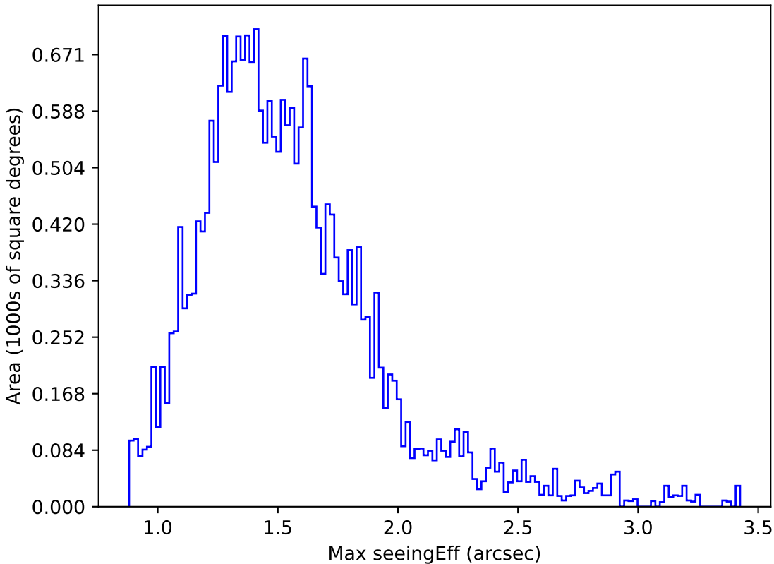
ddf_loaded_half_fl4_v3.4_10yrs Yr 1 g band: Max seeingEff
