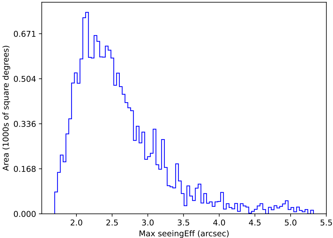
ddf_loaded_half_fl4_v3.4_10yrs WFD z band: Max seeingEff
