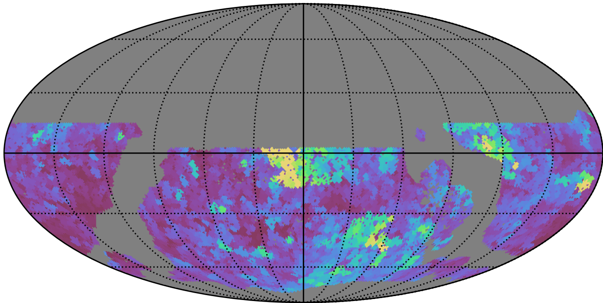
ddf_loaded_half_fl4_v3.4_10yrs WFD y band: Max seeingEff
