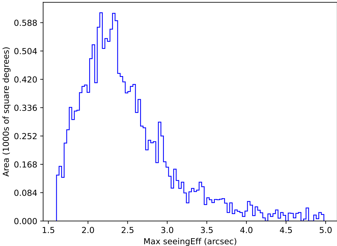
ddf_loaded_half_fl4_v3.4_10yrs WFD y band: Max seeingEff
