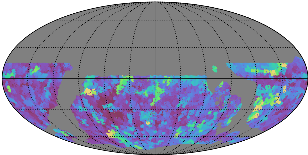
ddf_loaded_half_fl4_v3.4_10yrs WFD r band: Max seeingEff
