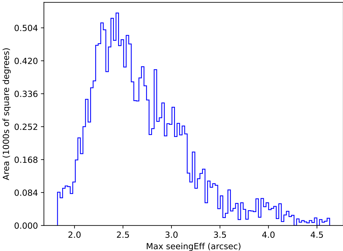
ddf_loaded_half_fl4_v3.4_10yrs WFD r band: Max seeingEff
