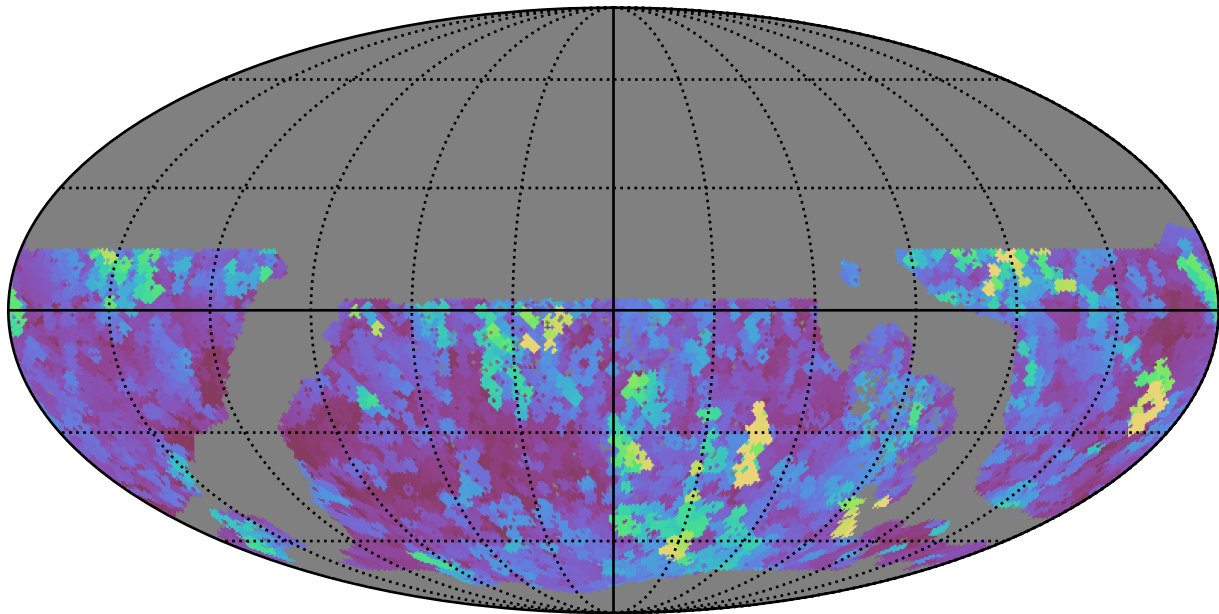
ddf_loaded_half_fl4_v3.4_10yrs WFD i band: Max seeingEff
