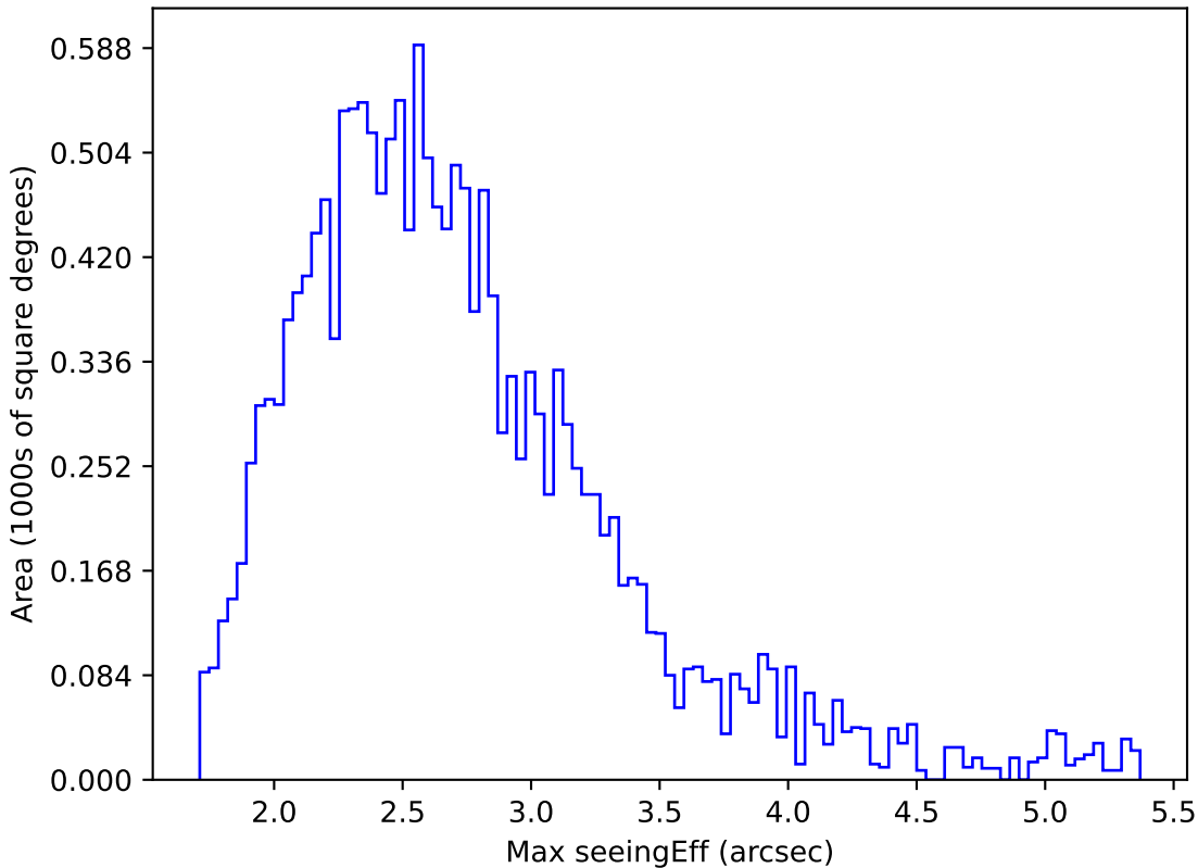
ddf_loaded_half_fl4_v3.4_10yrs WFD i band: Max seeingEff
