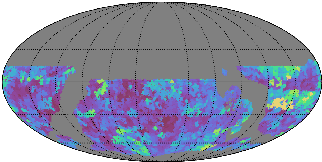
ddf_loaded_half_fl4_v3.4_10yrs WFD g band: Max seeingEff
