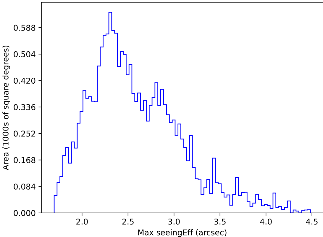
ddf_loaded_half_fl4_v3.4_10yrs WFD g band: Max seeingEff
