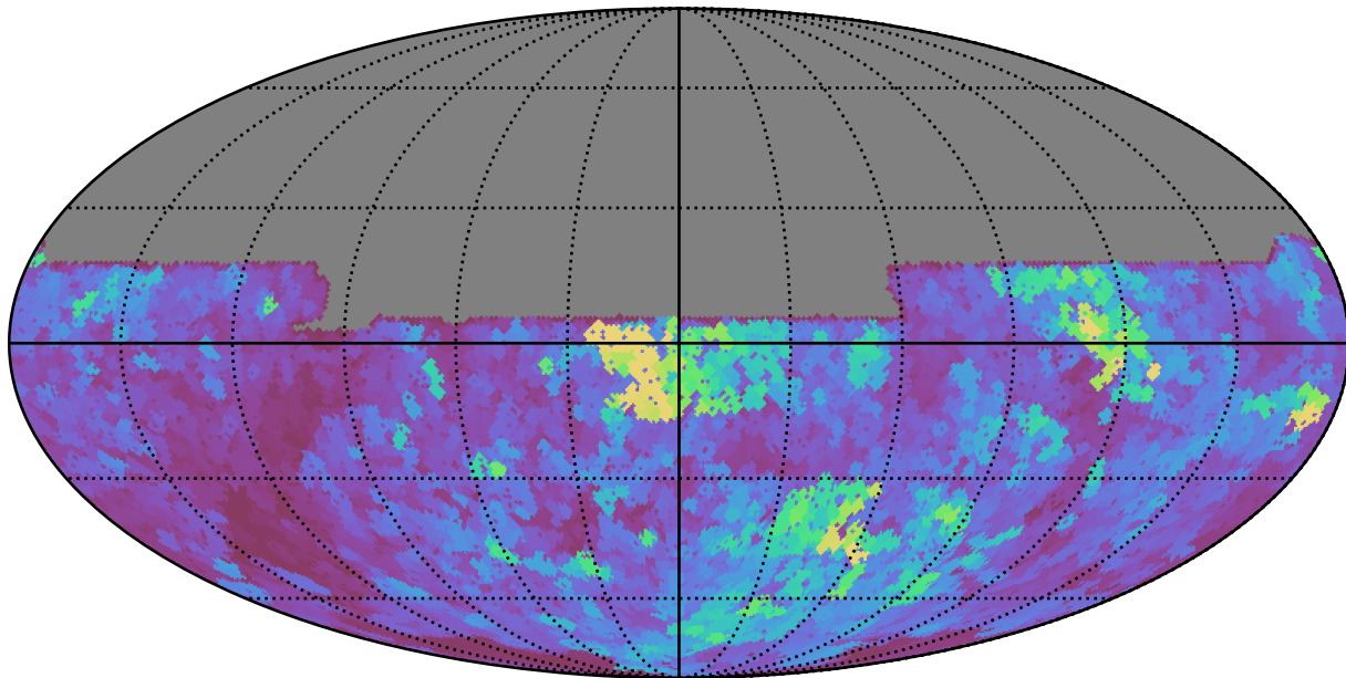
ddf_loaded_half_f14_v3.4_10yrs All sky y band: Max seeingEff
