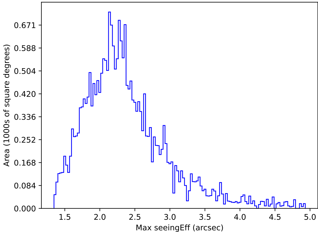
ddf_loaded_half_fl4_v3.4_10yrs All sky y band: Max seeingEff
