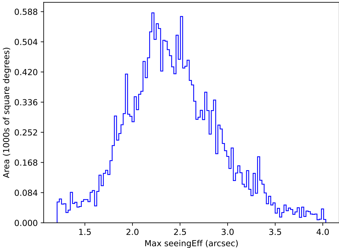
ddf_loaded_half_f14_v3.4_10yrs All sky u band: Max seeingEff
